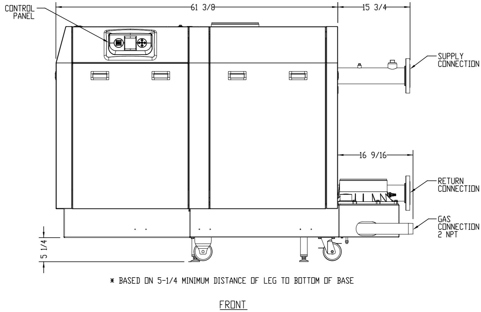
SLIMFIT SF1000 RH BOILER
